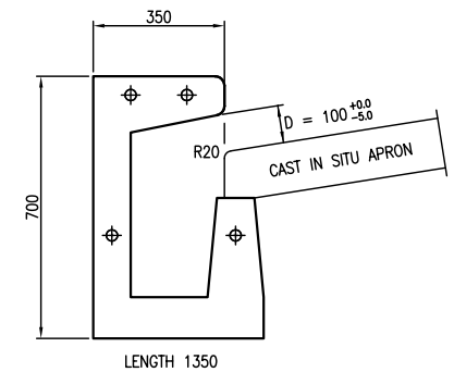
TROUGH AND APRON
