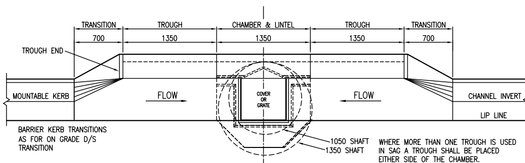
TYPICAL INLET IN SAG
