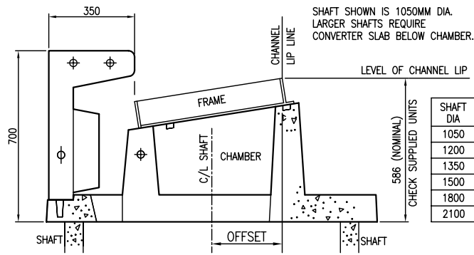
LINTEL, CHAMBER, FRAME AND SHAFT
