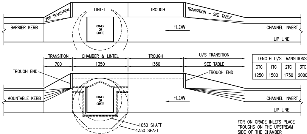
TYPICAL INLETS ON GRADE
